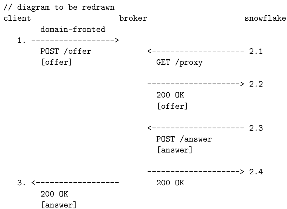
Figure 7.2: Snowflake rendezvous. The client makes only one HTTP request–response pair. In between the client’s request and response, the snowflake proxy makes two of its own request–response pairs, the first to learn the client’s offer and the second to send back its answer.
