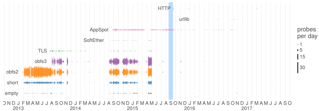
Figure 4.3: Active probes received at my web server over five years. This is an updated version of Figure 8 from the paper “Examining How the Great Firewall Discovers Hidden Circumvention Servers” [56]; the vertical blue stripe divides old and new data. The “short” probes are those that looked random but did not provide enough data (20 bytes) for the obfs2 test; it is likely that they, along with the “empty” probes, are really obfs2, obfs3, or Tor probes that were truncated at the first ‘\0’ or ‘\n’ byte.
