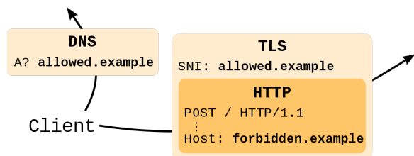
Figure 7.1: Domain fronting uses different names at different network layers.
